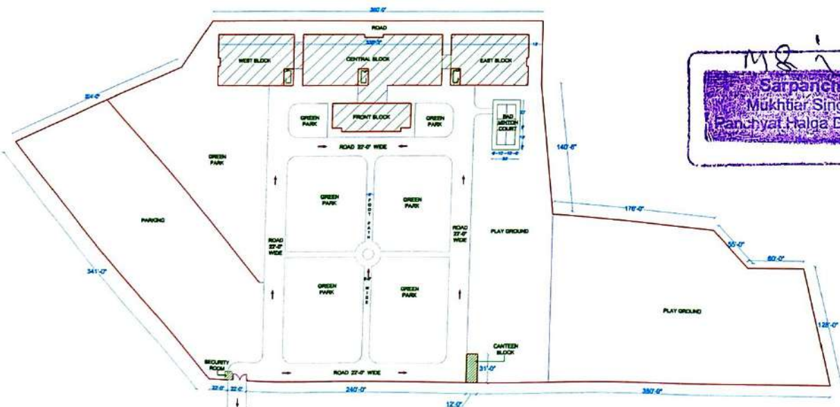
SITE PLAN
